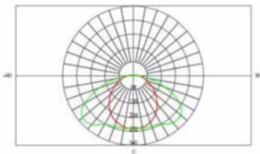
cd/1000 lm Curve
