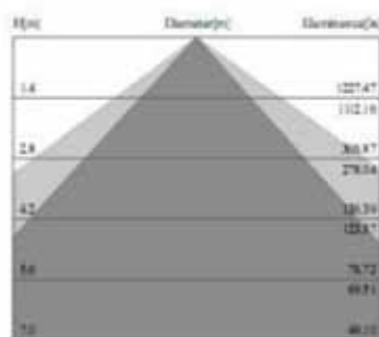
Illumination Cone Curve
