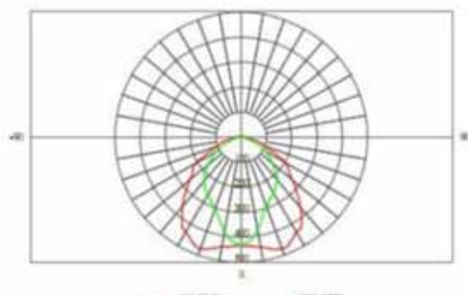
cd/1000 lm Curve
