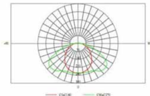
cd/1000 lm Curve
